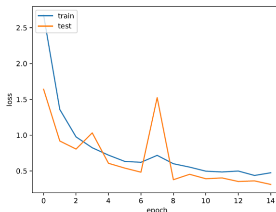
Figure 7. Loss vs. the number of epochs of CNN model predicted 10 classes without applying a feature extraction module.
