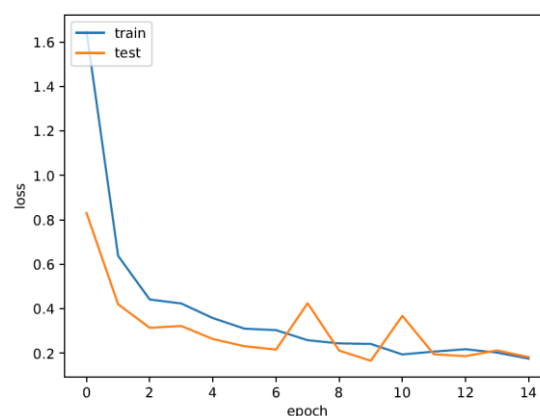
Figure 11. Loss vs. the number of epochs of CNN model predicted 10 classes with multi-triangles feature extraction module.
