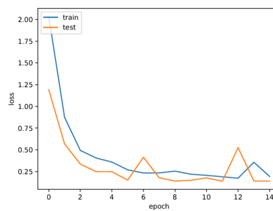
Figure 9. Loss vs. the number of epochs of CNN model predicted 10 classes with net-patterns feature extraction module.
