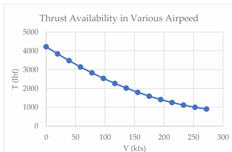
Figure 15. Thrust Availability
