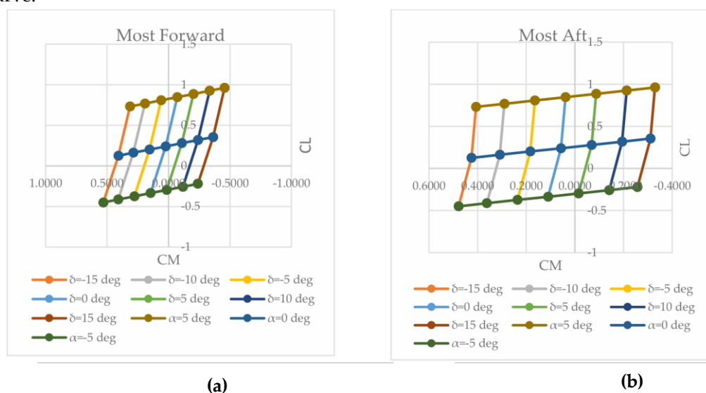
Figure 13. Trim Curve of \mathcal{A}\mathcal{E} -6 eLena Aircraft
