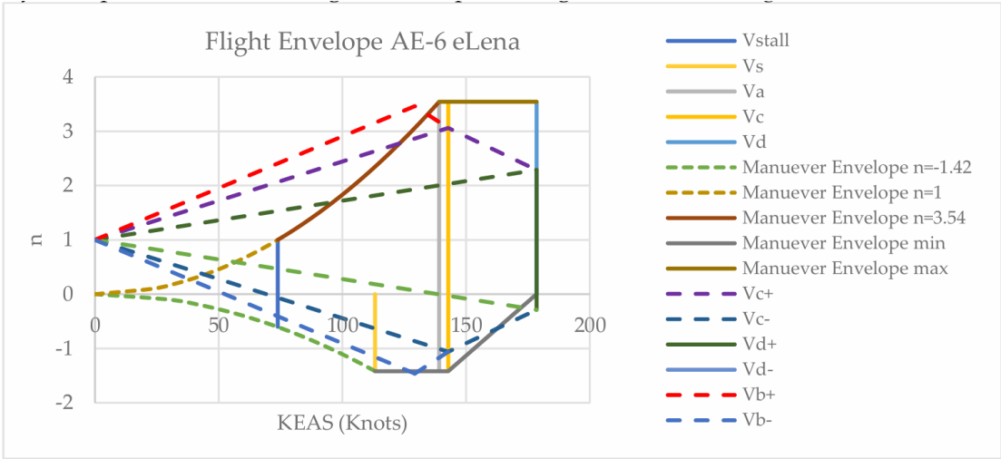
Figure 17. Flight Envelope
