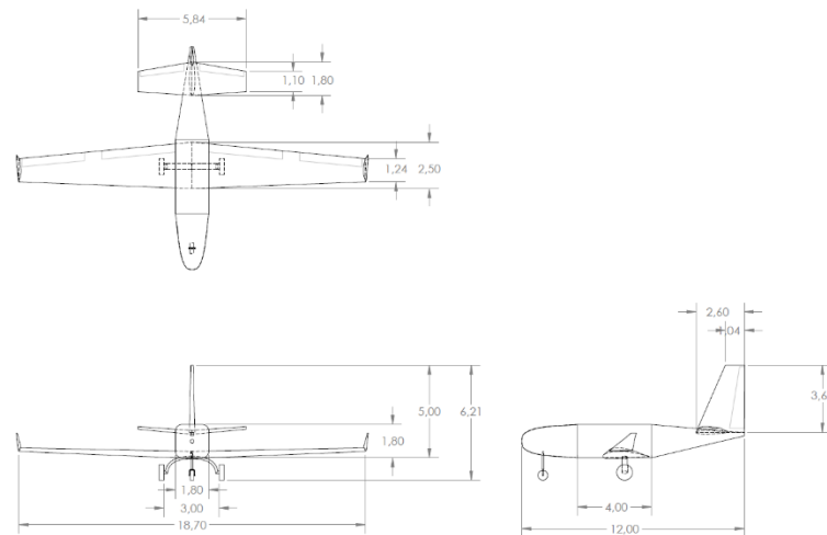
Figure 3. Aircraft Three-View Drawing
