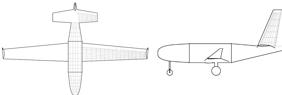
Figure 5. Structural Layout
