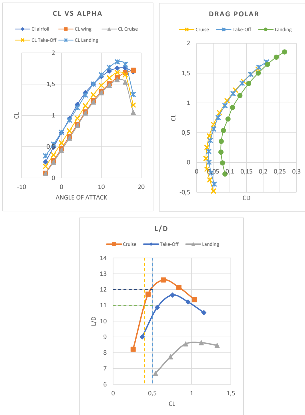
Figure 4. Aerodynamics Curves
