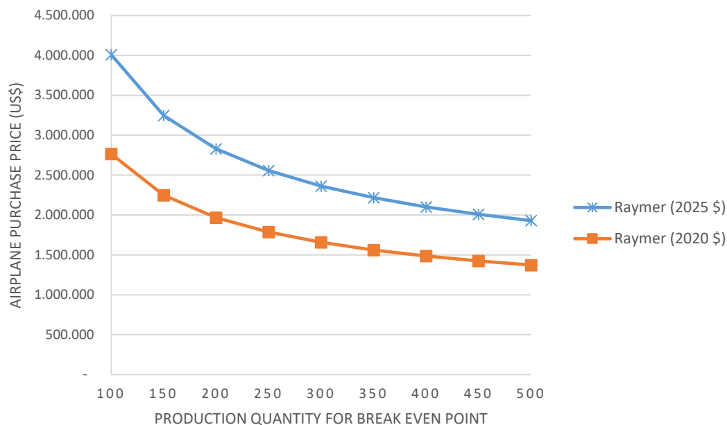
Figure 6. Estimation of Airplane Price and Break-Even Point
