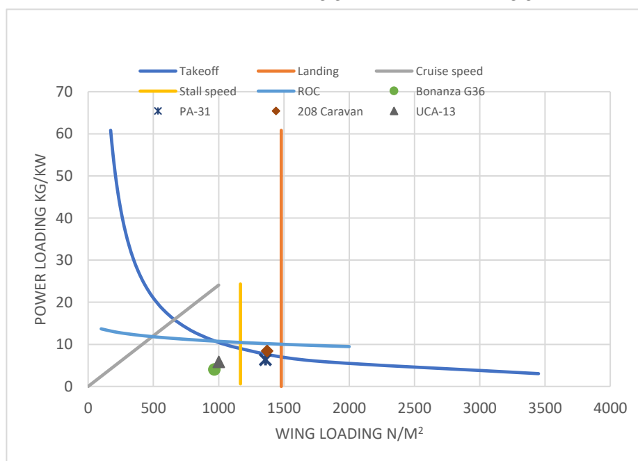
Figure 2. Matching Chart Estimation
