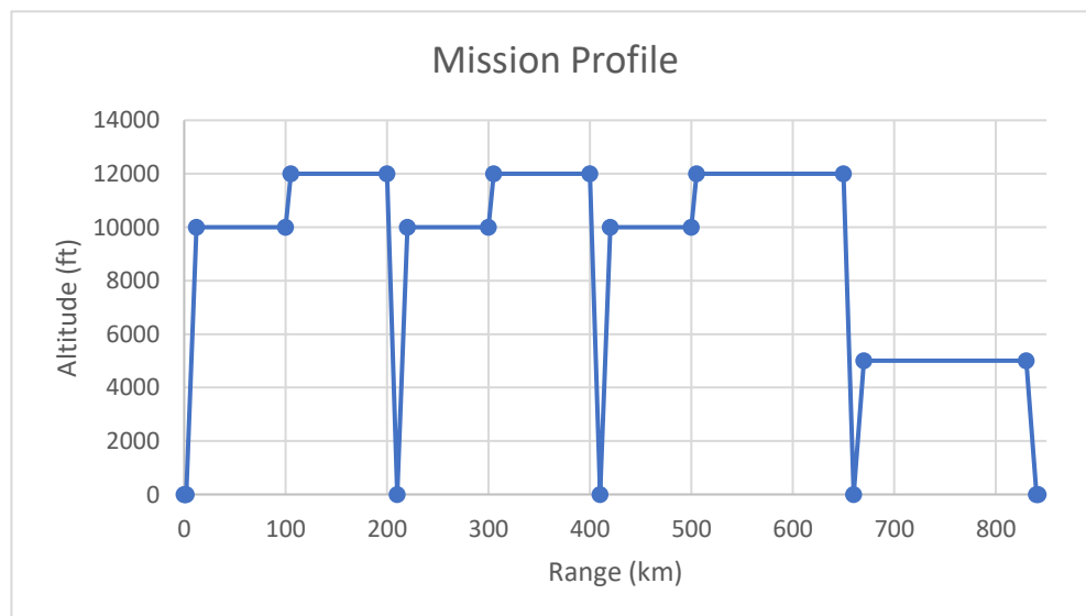
Figure 1. Mission Profile of UCA-13
