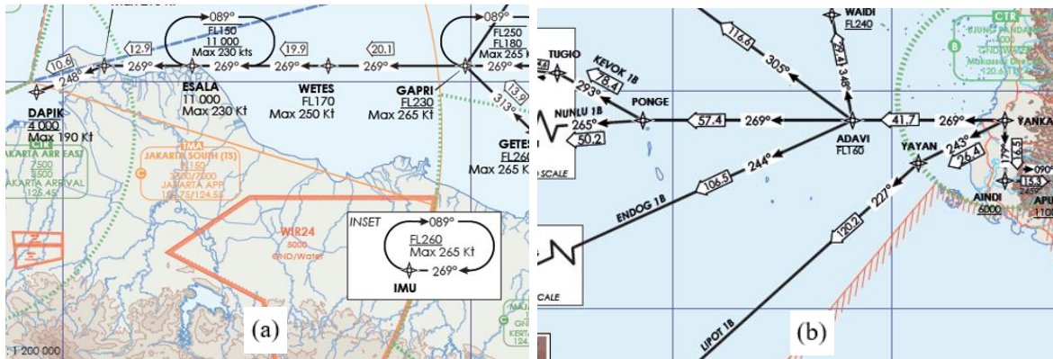
Figure 9. Published Flight Procedure for: (a) Arrival at Jakarta airport (CGK); (b) Departure at Makassar Airport (UPG)
