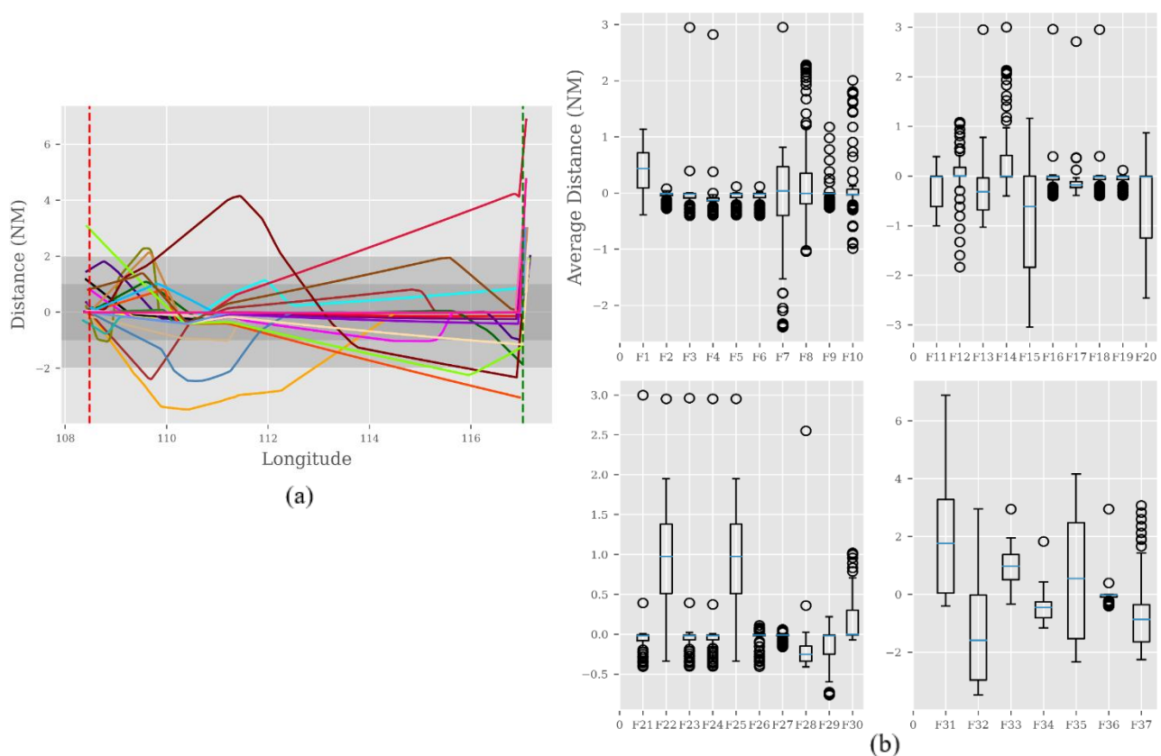
Figure 12. Deviation distance of Enroute segment: (a) Distance to Longitude; (b) Box plot of deviation distance of each flight data
