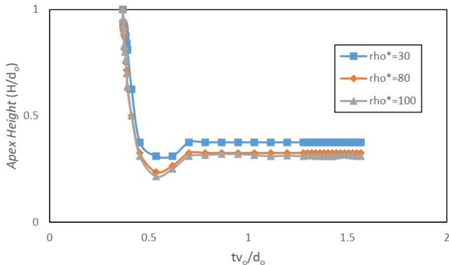
Figure 6. Non-dimensional diameter apex height in relation to (tv_o/d_o)
