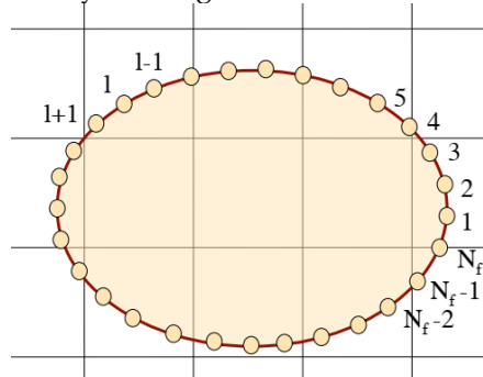
Figure 3. Marker points used to mark the interface between two fluids
