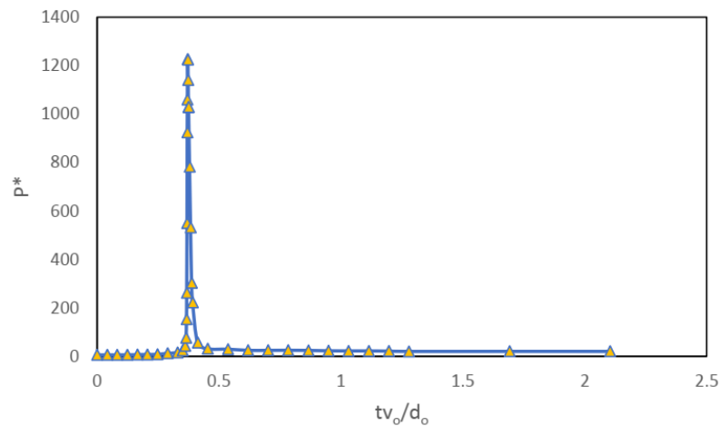
Figure 8. Pressure change as a function of time for a density ratio of 100.
