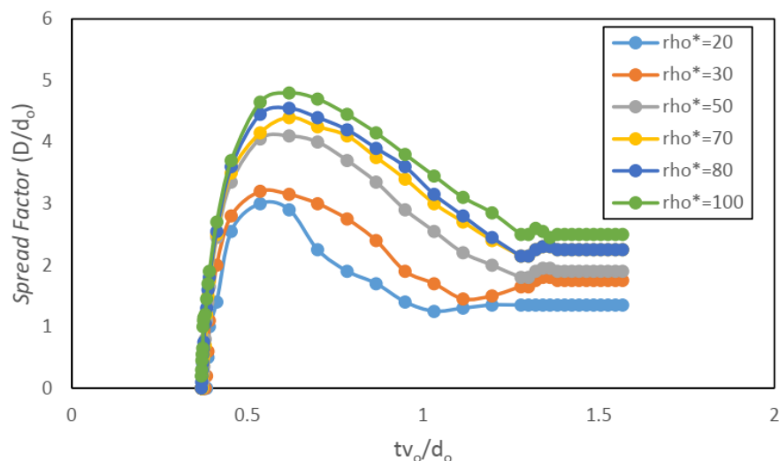
Figure 5. Non dimensional diameter spreading factor in relation to (tv_o/d_a)
