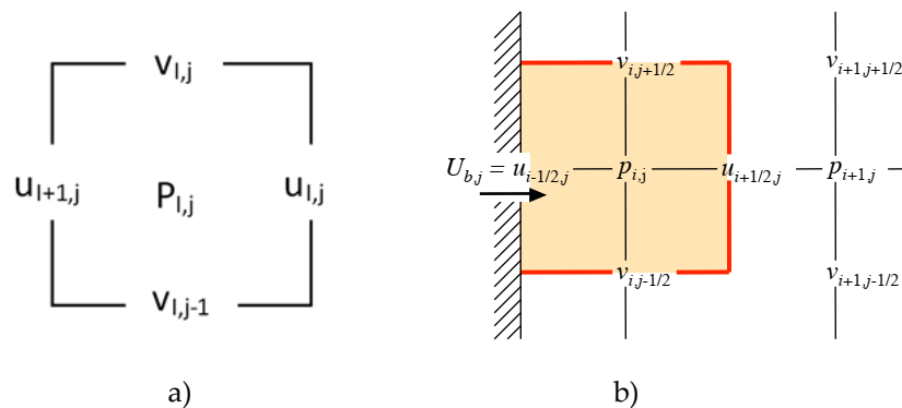
Figure 2. a) Computational domain in staggered-grid notation b) Boundary conditions
