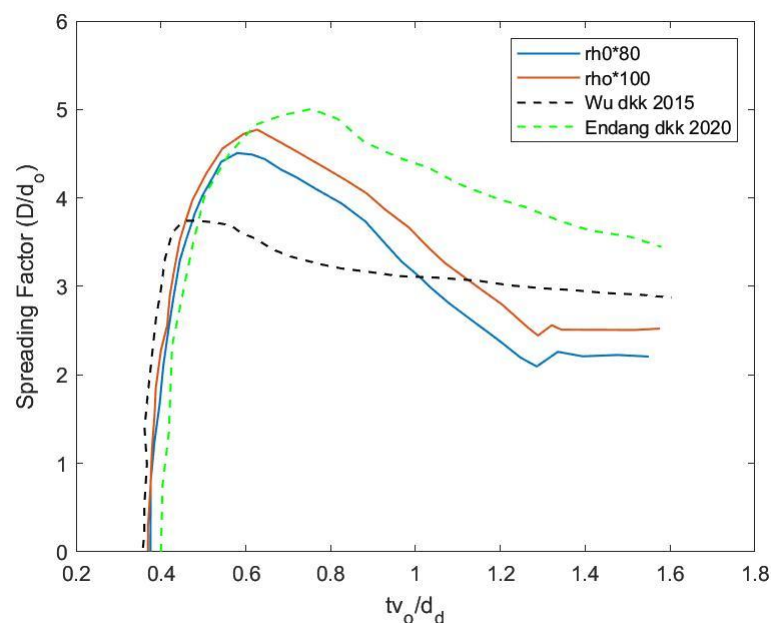
Figure 9. Comparison of the Spread Factor of this study ( Q^* = 80 , Q^* = 100 ) with data from Wu et al. (2015) [14] and Endang et al. (2020) [11].
