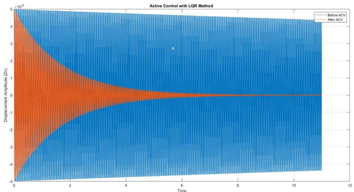
Figure 5. Implementation of Active Control Vibration on Spacecraft Structure with Linear Quadratic Regulator Method
