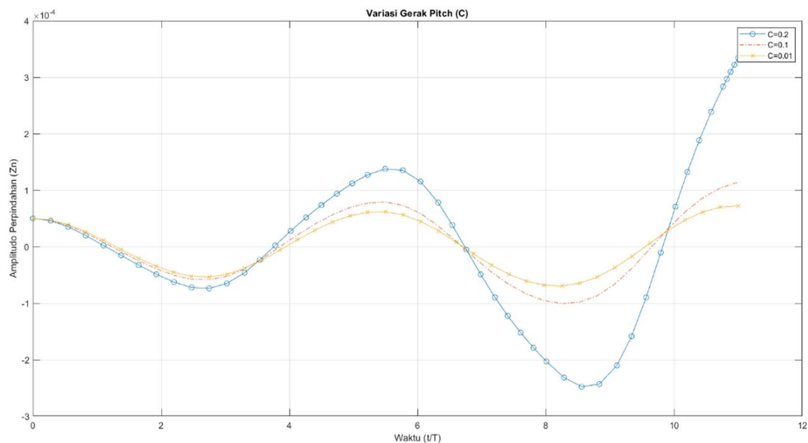
Figure 3. Structural Response due to Variation of Spacecraft Pitch Angle
