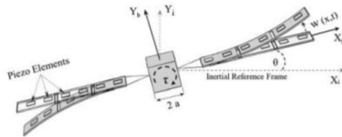
Figure 1. Illustration of Spacecraft with Flexible Solar Panel Structure [3]
