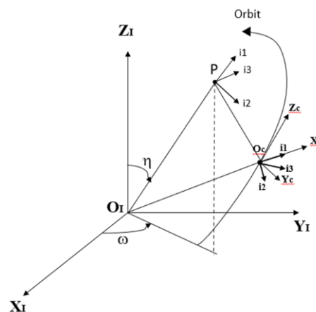
Figure 2. Integrated Coordinate Reference System
