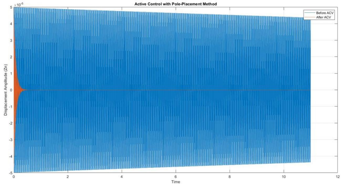
Figure 4. Implementation of Active Control Vibration on Spacecraft Structure with Pole-Placement Method
